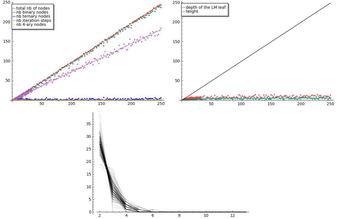
Figure 7.3: Simulation of different parameters on Strict monotonic Schröder trees . (left) The number of d -ary nodes and the number of iteration steps. (right) The height and the depth of the (LM) leftmost leaf. The sizes of the sampled trees range from 1 to 250. (down) Root degree, the lines gets darker as n moves from 2 to 100, with 40 trees sampled for each size.
