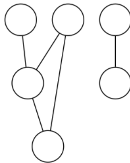
Figure 3.6: A graph of 6 vertices
