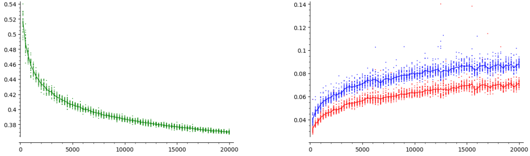
Figure 6.9: (left) Experimental compression ratio; (right) Experimental search time comparison
