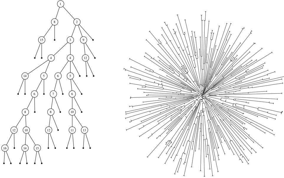
Figure 4.9: Two strict monotonic Schröder trees
