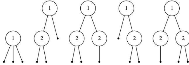
Figure 4.17: All strict monotonic general Schröder trees of size 3
