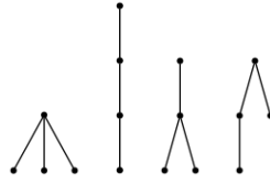
Figure 3.11: All 4 Pólya trees of size 4.
