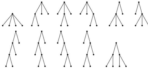
Figure 3.12: All 11 Schröder trees of size 4.
