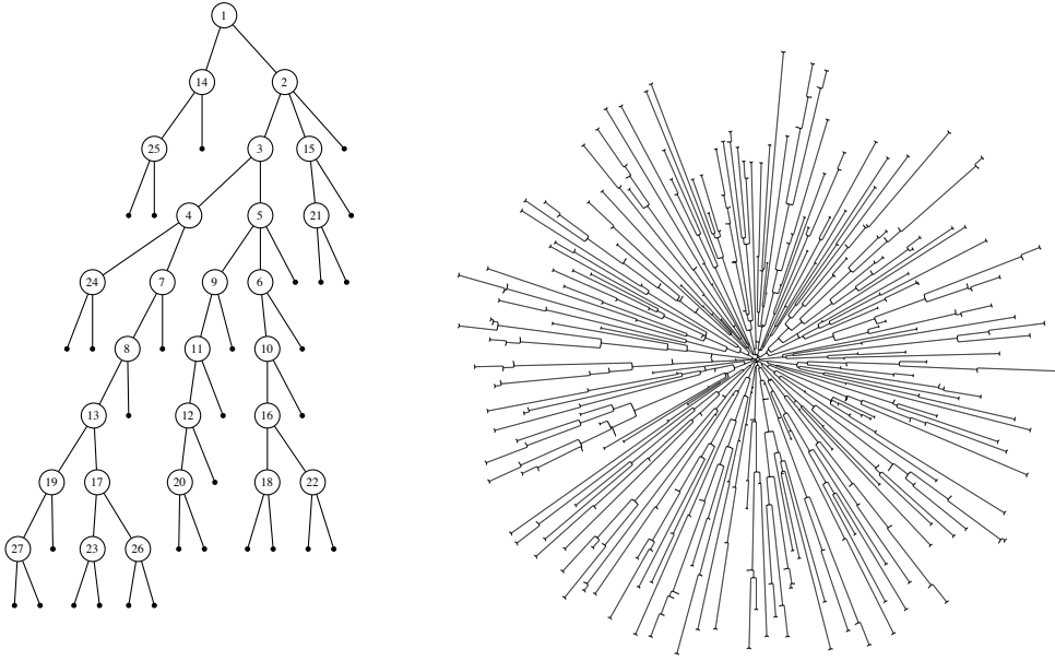
Figure 4.2: Two increasing Schröder trees
