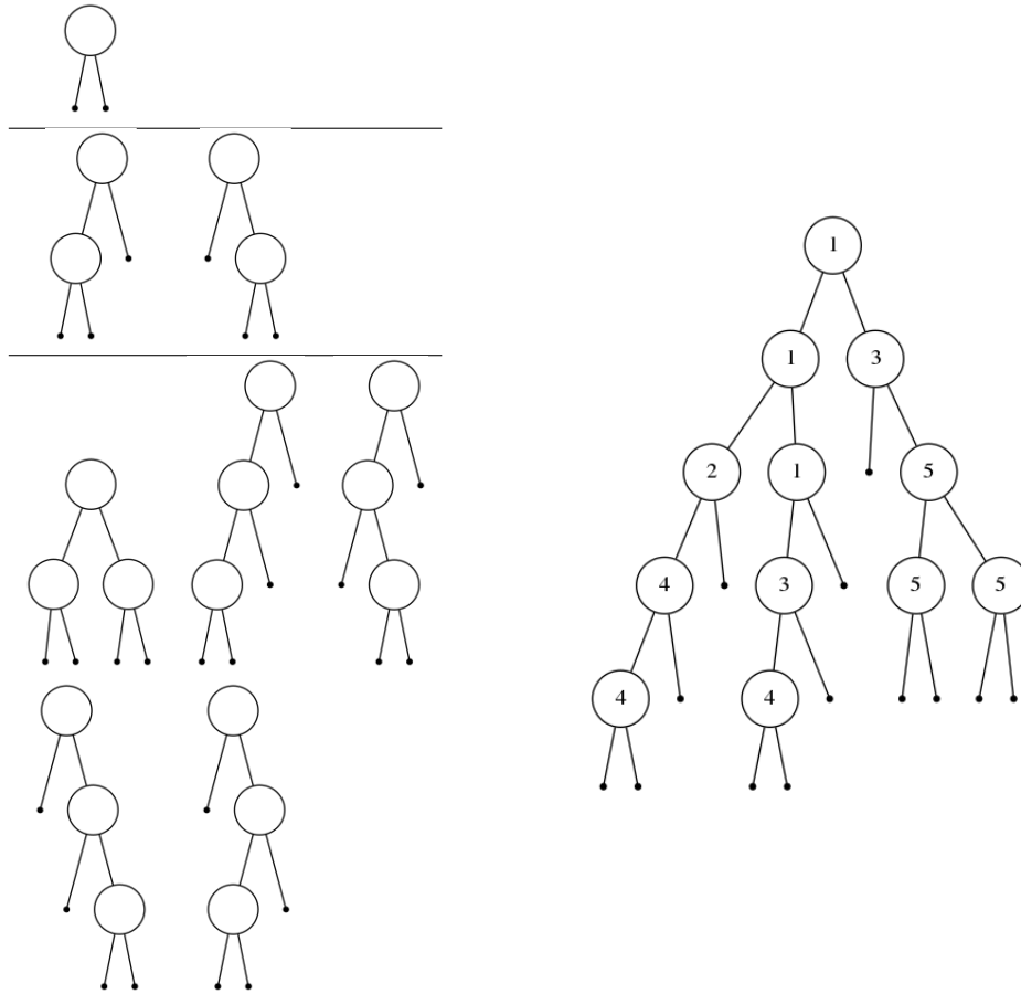
Figure 5.2: Example of Definition 5.3.1 . (Left) An example of the colored degree function, seen as a class of rooted unlabelled trees here binary trees \phi(z) = z^2 + 2z^3 + 5z^4 , the trees of first sizes 2, 3 and 4 are depicted. At each iteration step a leaf can evolve into a whole unlabelled shape and that all its internal nodes get the label of the current iteration step. (Right) A resulting monotonic binary tree, here r = \mathbb{N}^* .
